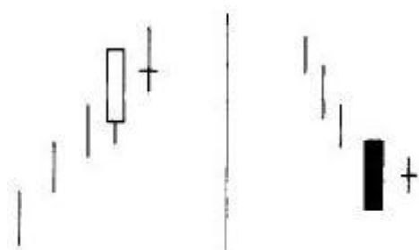
EXHIBIT 6.3. Harami Cross
