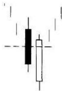
EXHIBIT 4.29. Piercing Pattern
