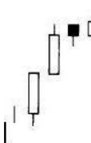
EXHIBIT 6.58. Tower Top
