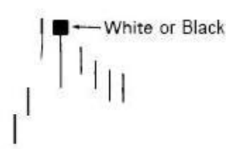
EXHIBIT 4.6. Hanging Man
