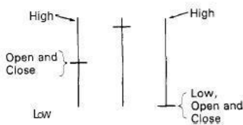
EXHIBIT 3.7. Doji Examples
