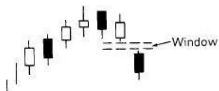
EXHIBIT 6.53. Dumping Top
