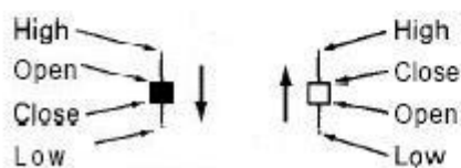
EXHIBIT 3.6. Spinning Tops
