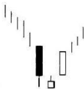
EXHIBIT 5.3. Morning Star
