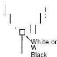
EXHIBIT 4.5. Hammer
