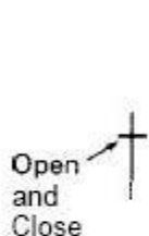
EXHIBIT 8.1. Doji
