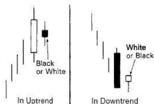
EXHIBIT 6.1. Harami
